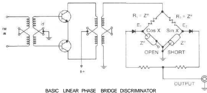
BASIC LINEAR PHASE BRIDGE DISCRIMINATOR
